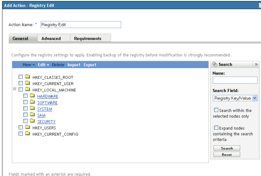
Figure 6-29 Action - Registry Edit Dialog Box: General Tab
